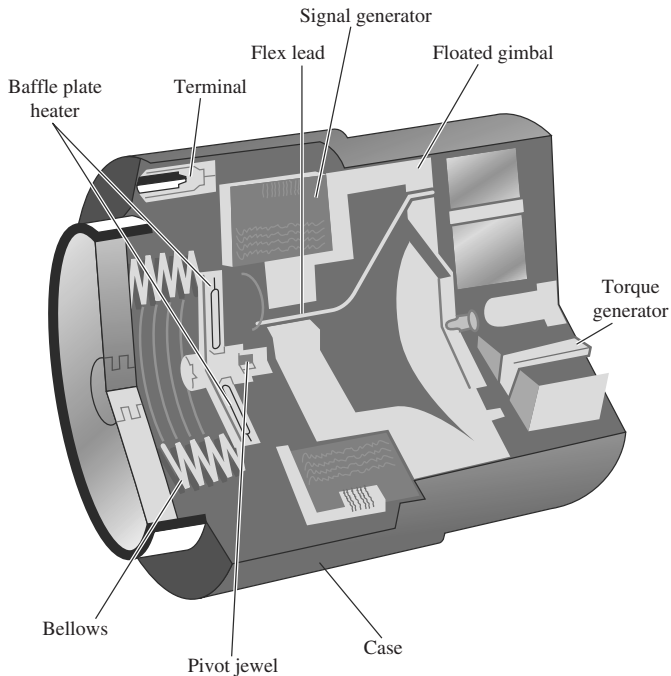
FIGURE 4-19 Cutaway view of an actual floated gimbal accelerometer. Based
