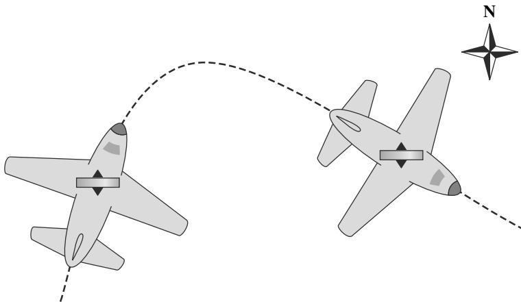
FIGURE 4-2 A directional gyroscope maintains its orientation in an airplane
