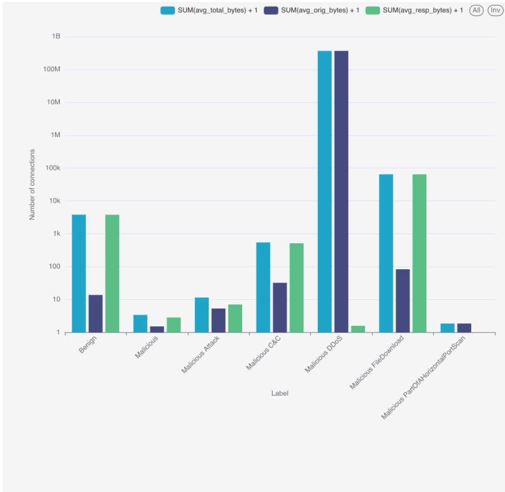
FIG. 03 · DDoS AVERAGES ≈ 3.7×10 8 ORIG BYTES / FLOW – SIX ORDERS OF MAGNITUDE OVER BENIGN. PORT-SCAN AND GENERIC MALICIOUS CARRY < 1B PER CONNECTION ON AVERAGE.
