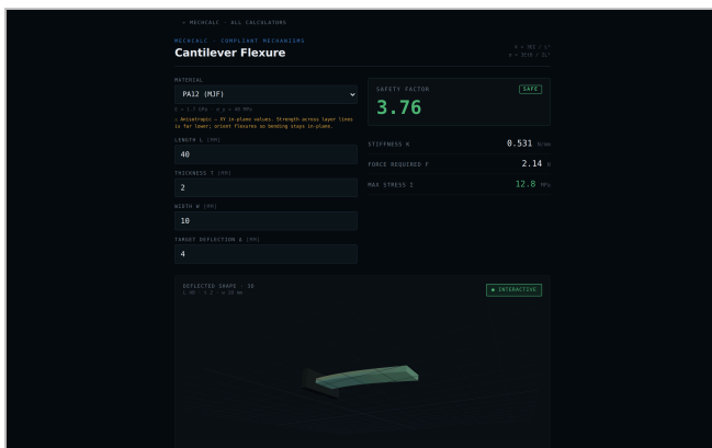
Fig. 2a — Same tool, first parameter set. A PA12 (MJF-printed) blade, 40 × 10 × 2 mm, asked for 4 mm of deflection: safety factor 3.76, SAFE.
