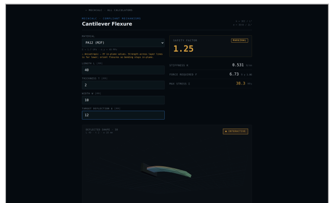
Fig. 2b — Second parameter set. The same blade asked for 12 mm: the factor drops to 1.25 and turns MARGINAL, the force readout picks up an uncertainty factor, and the beam's colors shift toward the loaded root.
