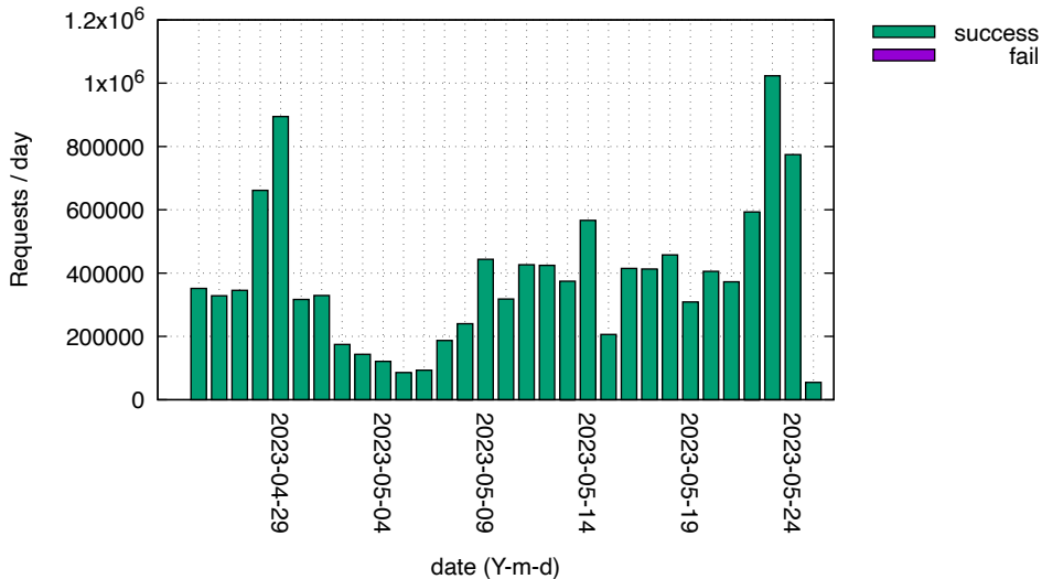
HTTP PROPFIND requests on CMS dCache daily
