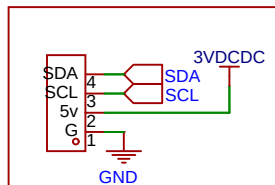
I2c bus connector
