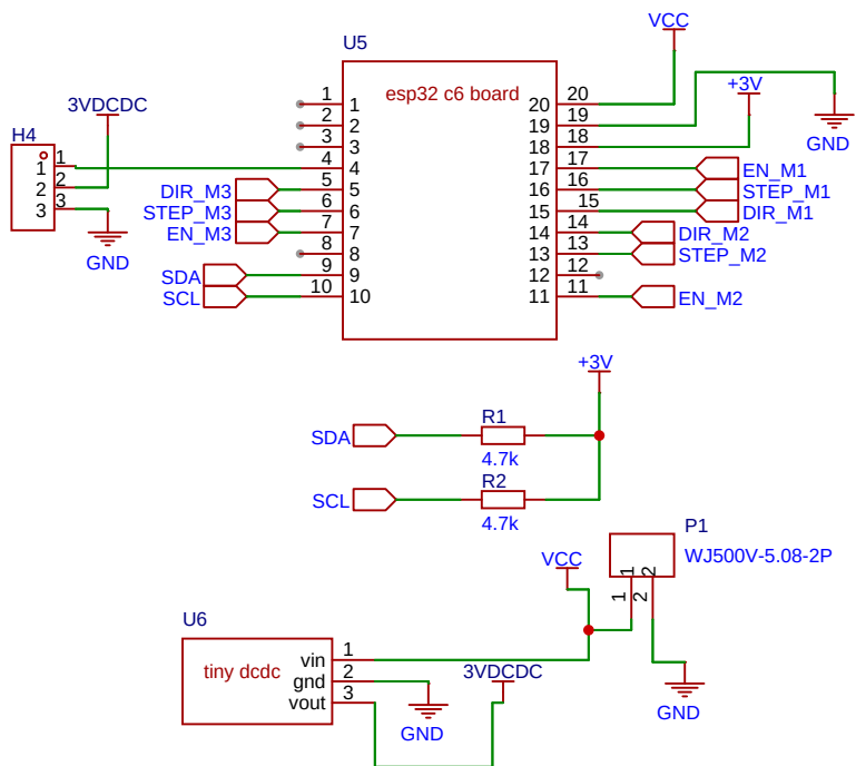
I2c bus connector
