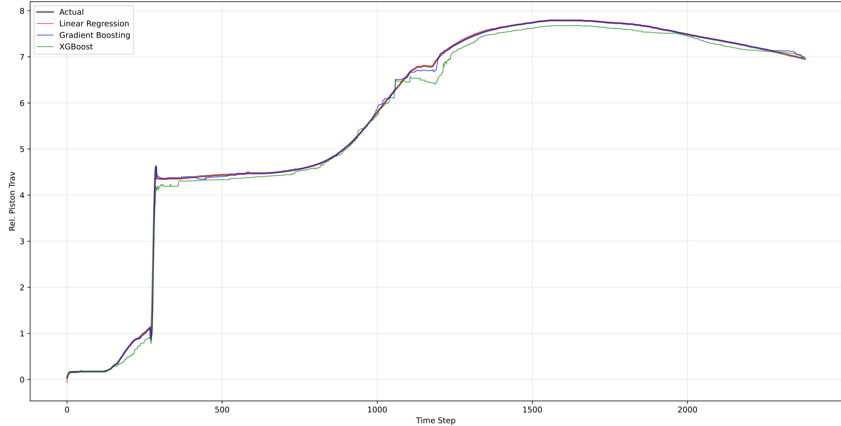
Top 3 Models Comparison
