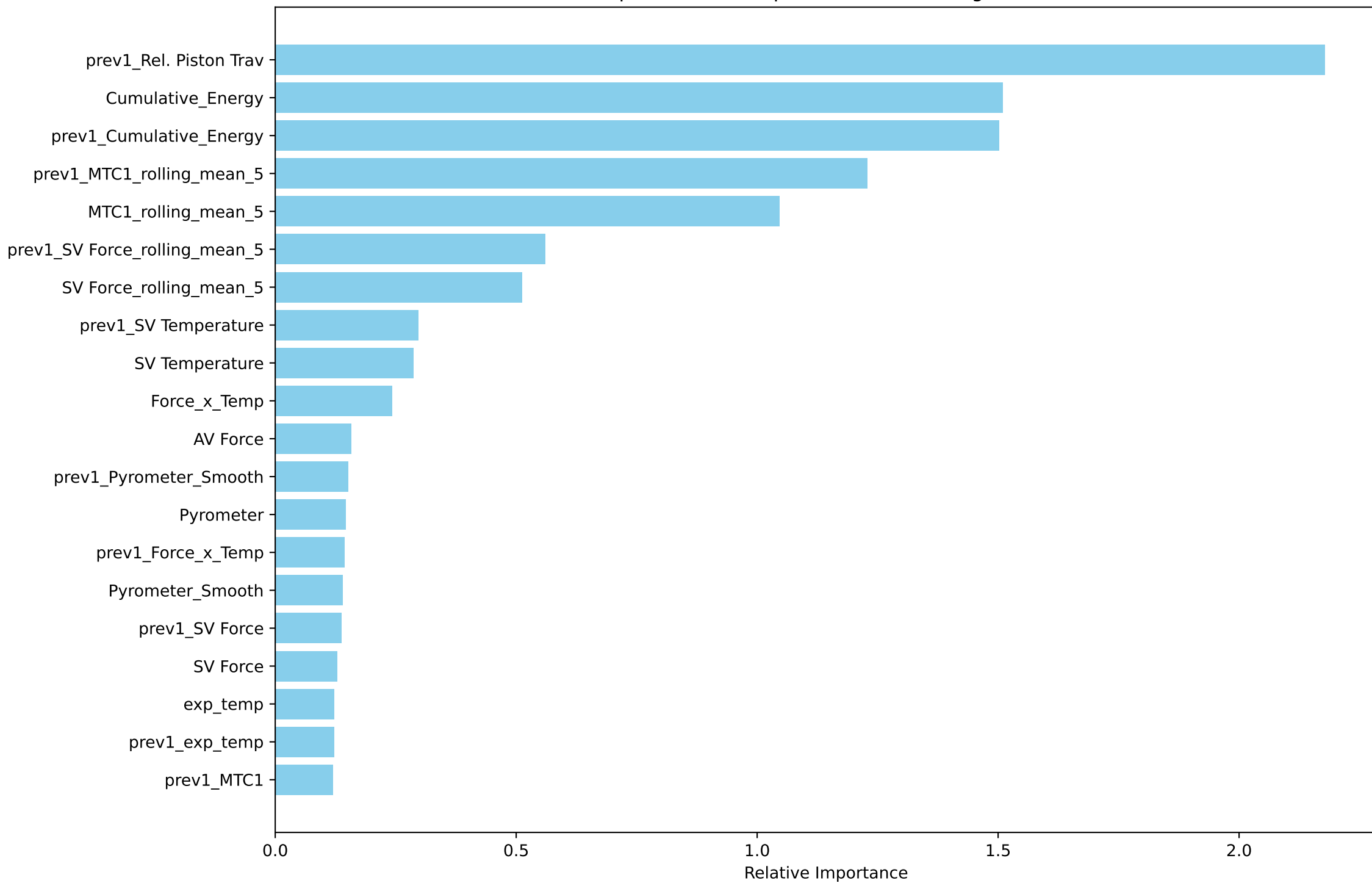
Top 20 Feature Importance - Linear Regression
