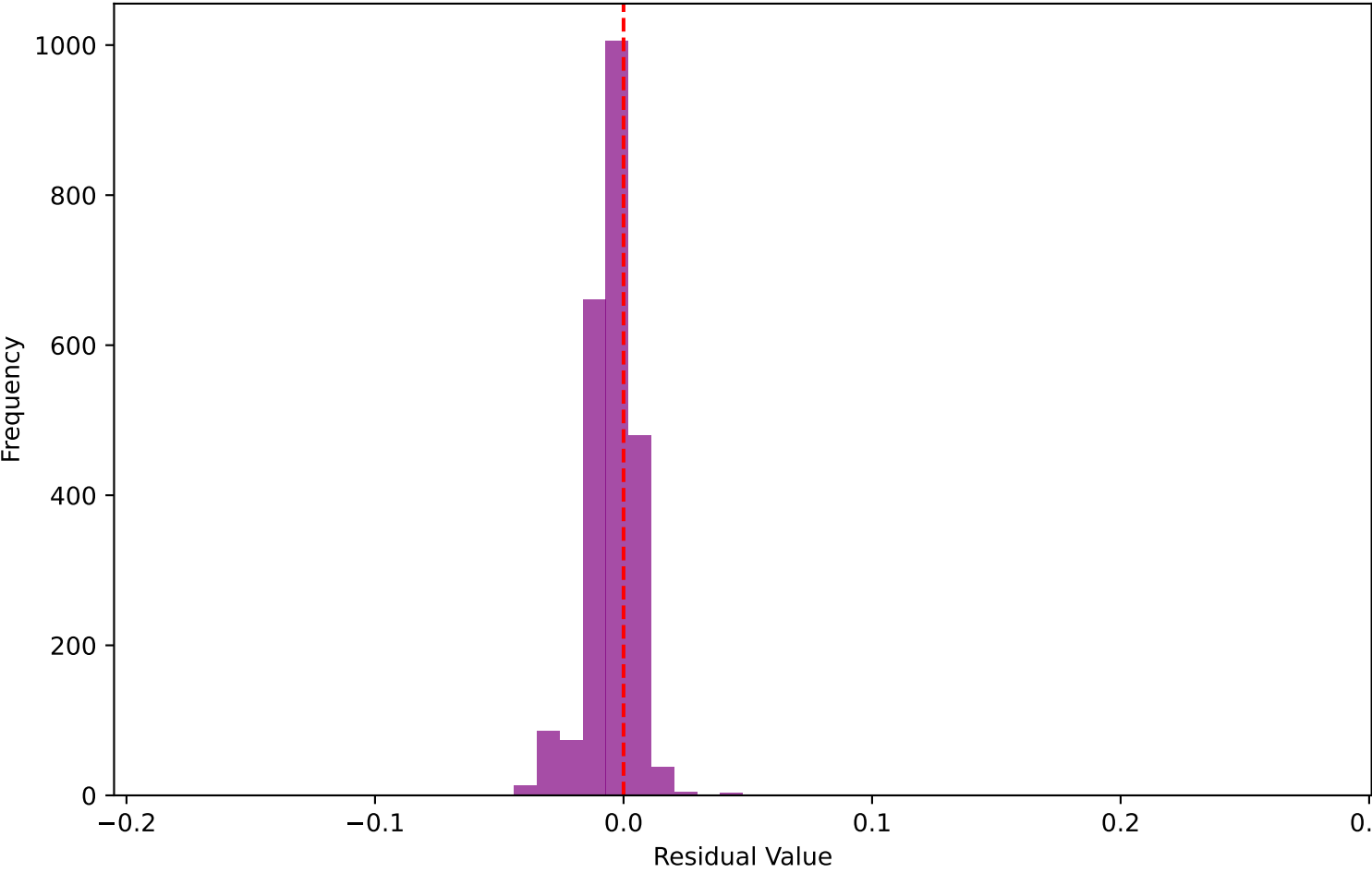
Residual Distribution
