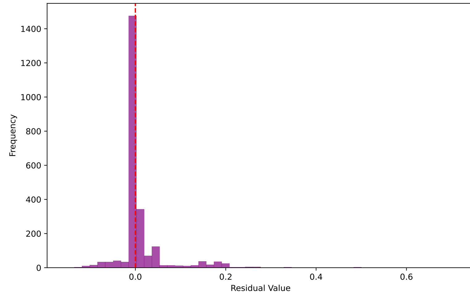
Residual Distribution
