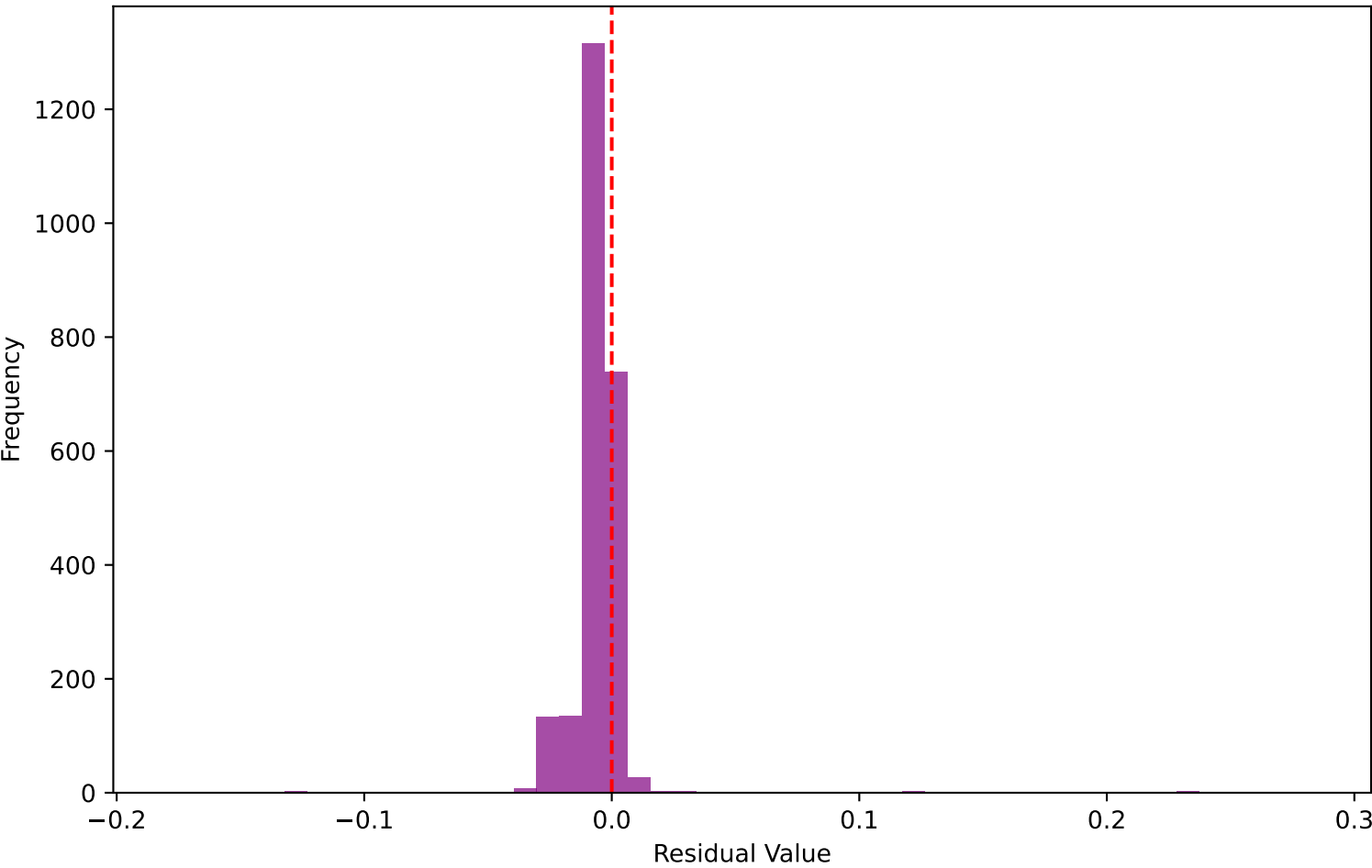
Residual Distribution
