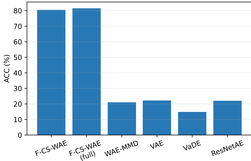
Available CIFAR-10 Accuracy
