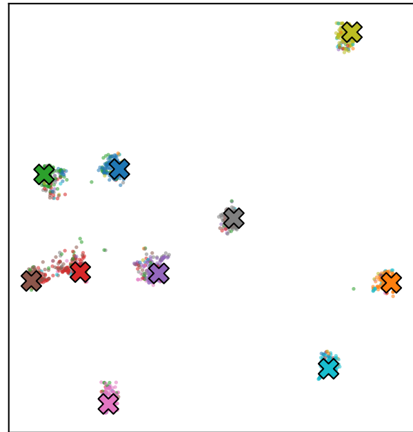
F-CS-WAE z_c
