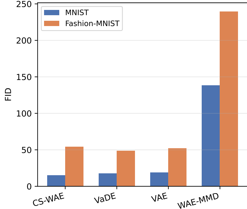
Fréchet Inception Distance
