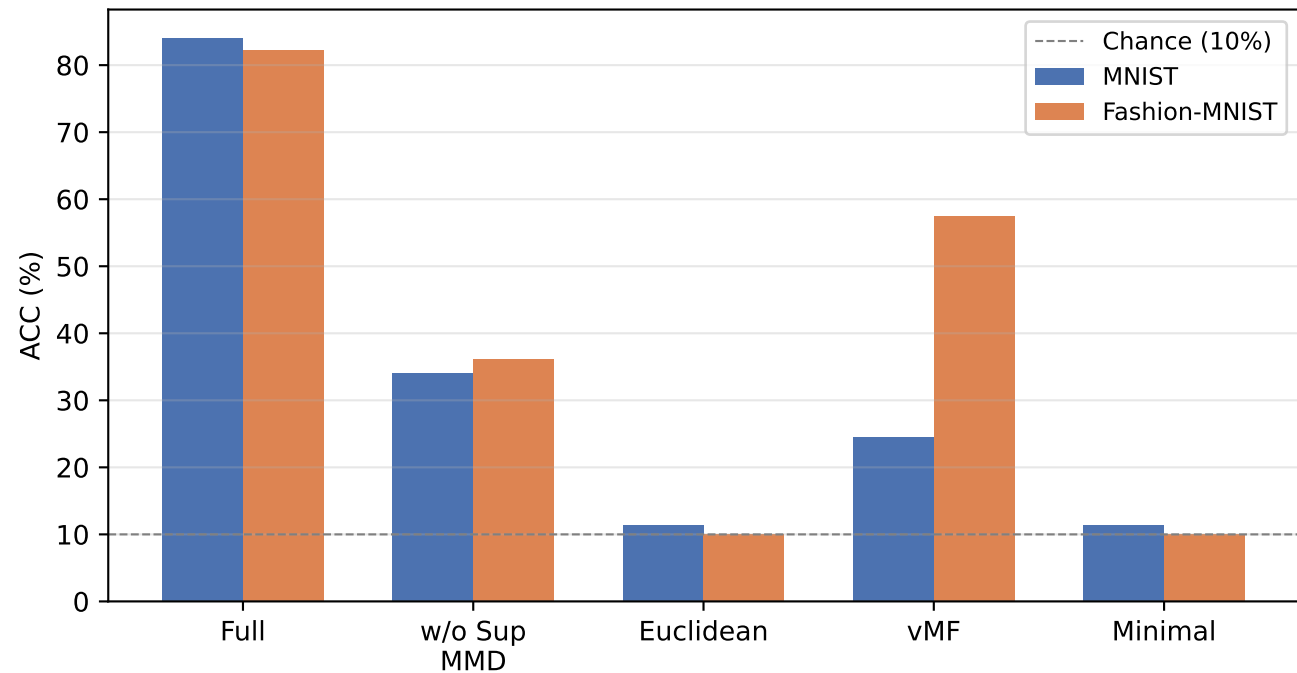
Ablation Study — Clustering Accuracy (seed 0)
