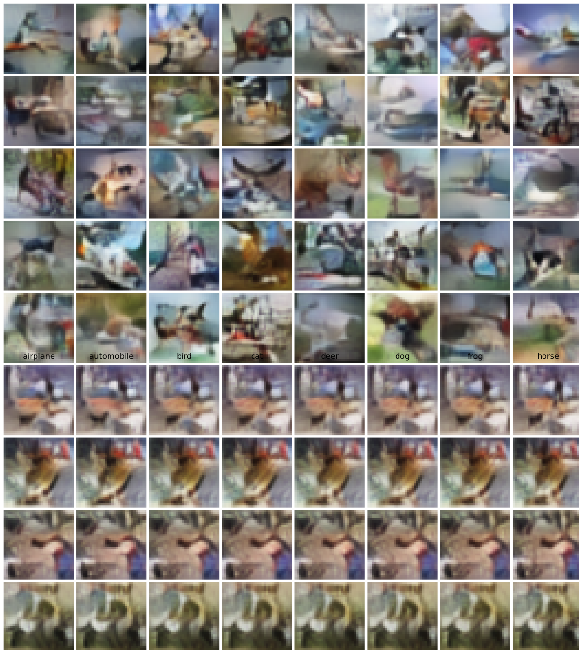
Figure 4: CIFAR-10 factorization probe. Columns: fixed z_c , varying z_s . Rows: fixed z_s , varying z_c .
