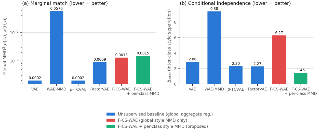
Figure 1: Global MMD (panel a, log scale) vs. inter-class style separation \Delta_{\text{inter}} (panel b) across the five model families and the per-class-style-MMD variant of F-CS-WAE (Table 1). Marginal matching quality (panel a) is not predictive of conditional independence (panel b).
