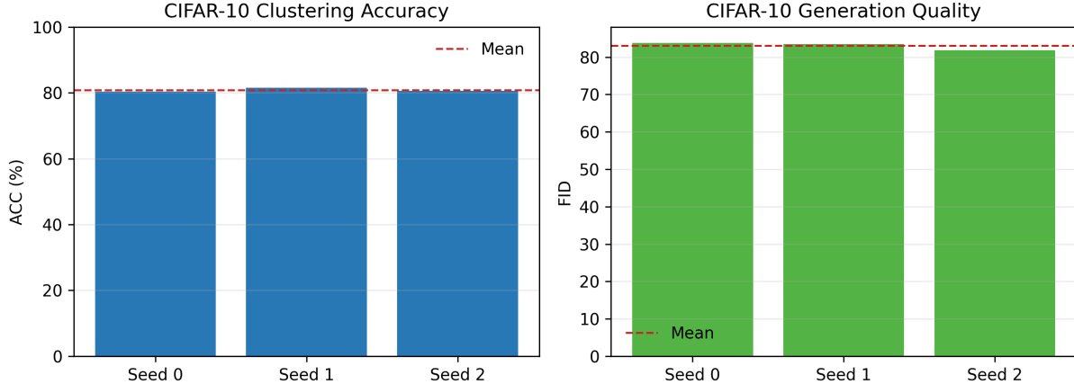
Figure 2: CIFAR-10 clustering and FID across three F-CS-WAE seeds. Variance is low.
