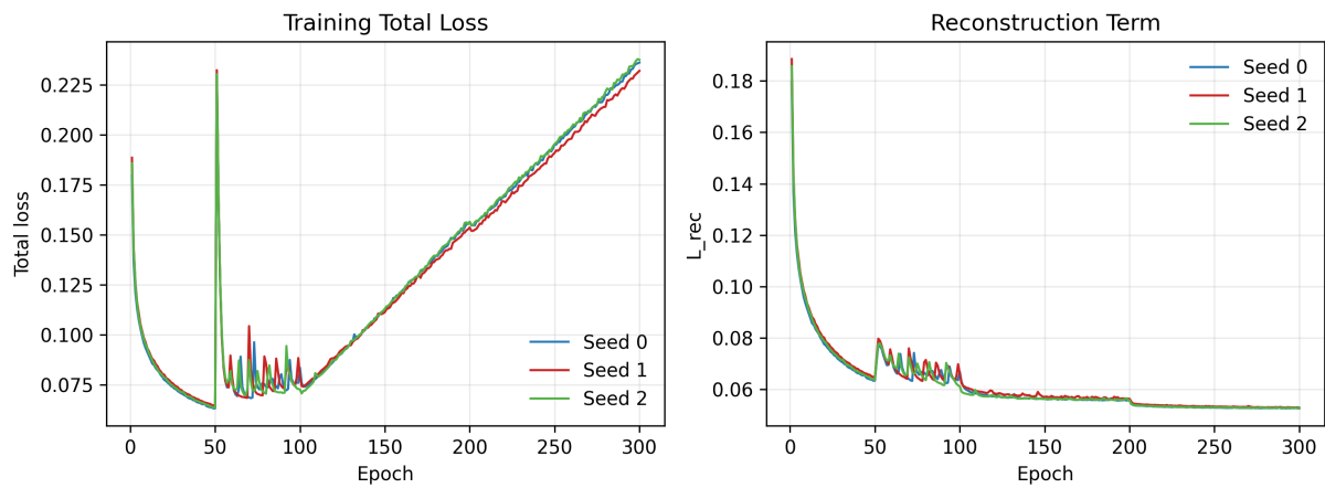
Figure 5: CIFAR-10 training curves. Phase transitions at epochs 50, 100, 200.
