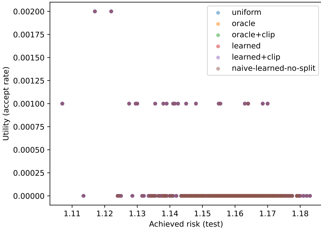
Utility vs risk (Exp1)
