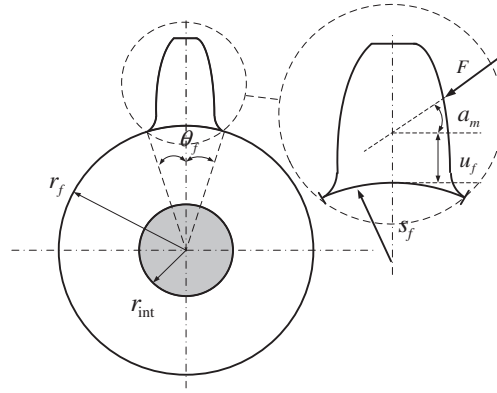
Fig. 2. Geometrical parameters for the fillet-foundation deflection.
