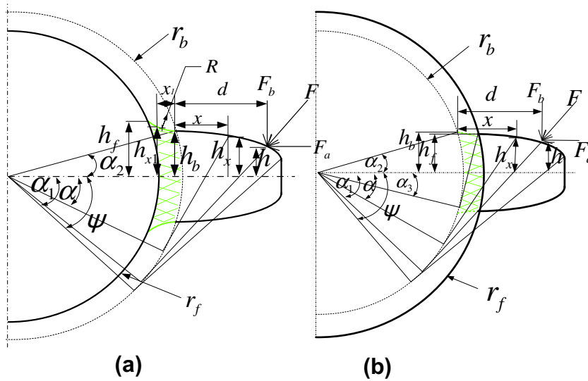
Fig. 3. Schematic of spur gear when z < 42 (a) and z > 42 (b).
