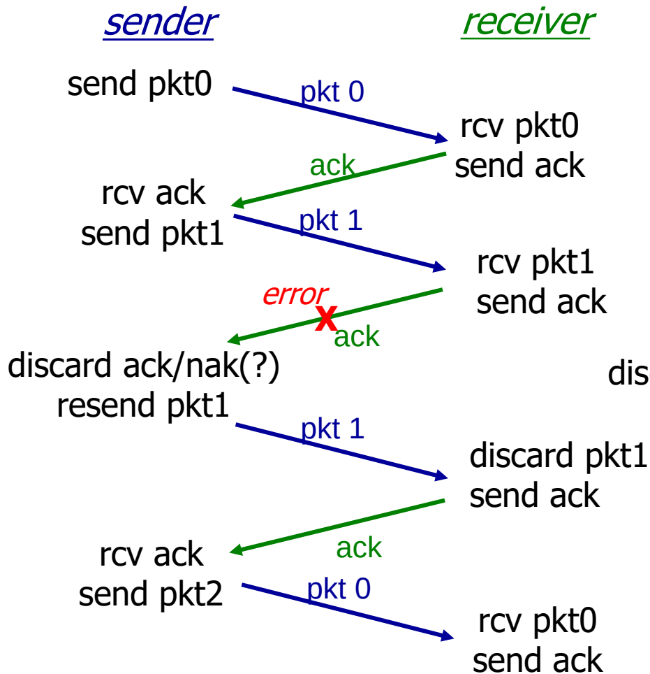
(a) ACK error
