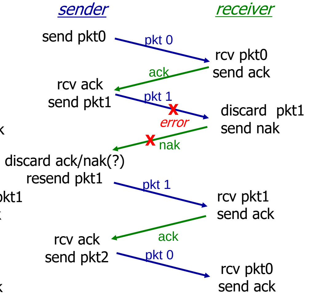
(b) packet and NAK error
