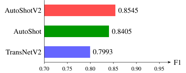
Fig. 3. F1-score comparison on SHOT. AutoShotV2 improves the reproduced AutoShot baseline by 1.40% and the reported TransNetV2 baseline by 5.52% in absolute F1.
