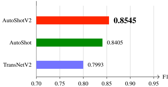
Fig. 3. F1-score comparison on SHOT. AutoShotV2 improves the reproduced AutoShot baseline by 1.40 points and the reported TransNetV2 baseline by 5.52 points.
