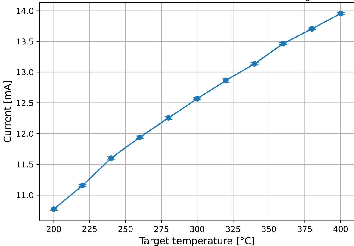
Current consumption as a function of T_{target}
