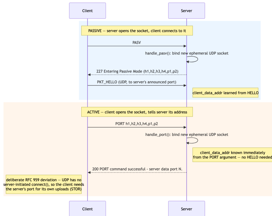
Figure 2: Passive (PASV) vs. Active (PORT) mode negotiation.
