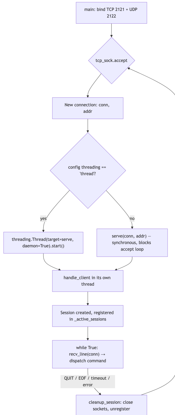
Figure 3: Server thread-dispatch logic.
