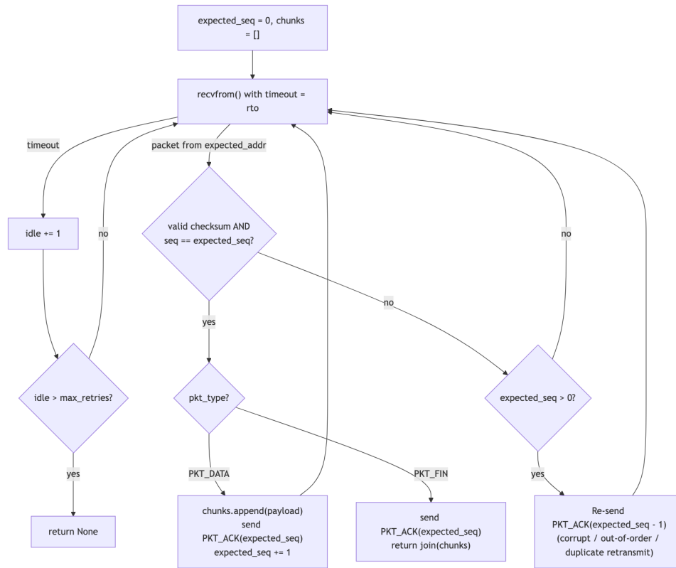
Figure 5: Go-Back-N receiver state machine. Only strictly in-order packets are accepted and buffered; anything else re-triggers the last known-good cumulative ACK.
