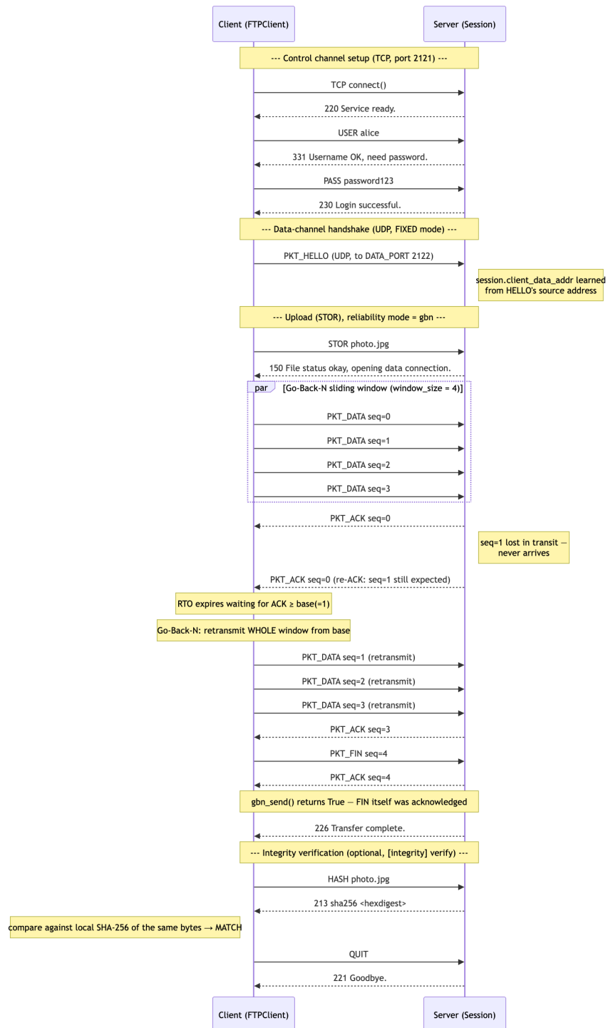
Figure 1: Full TCP + UDP session lifecycle, including a Go-Back-N retransmission after a simulated packet loss on seq=1 .
