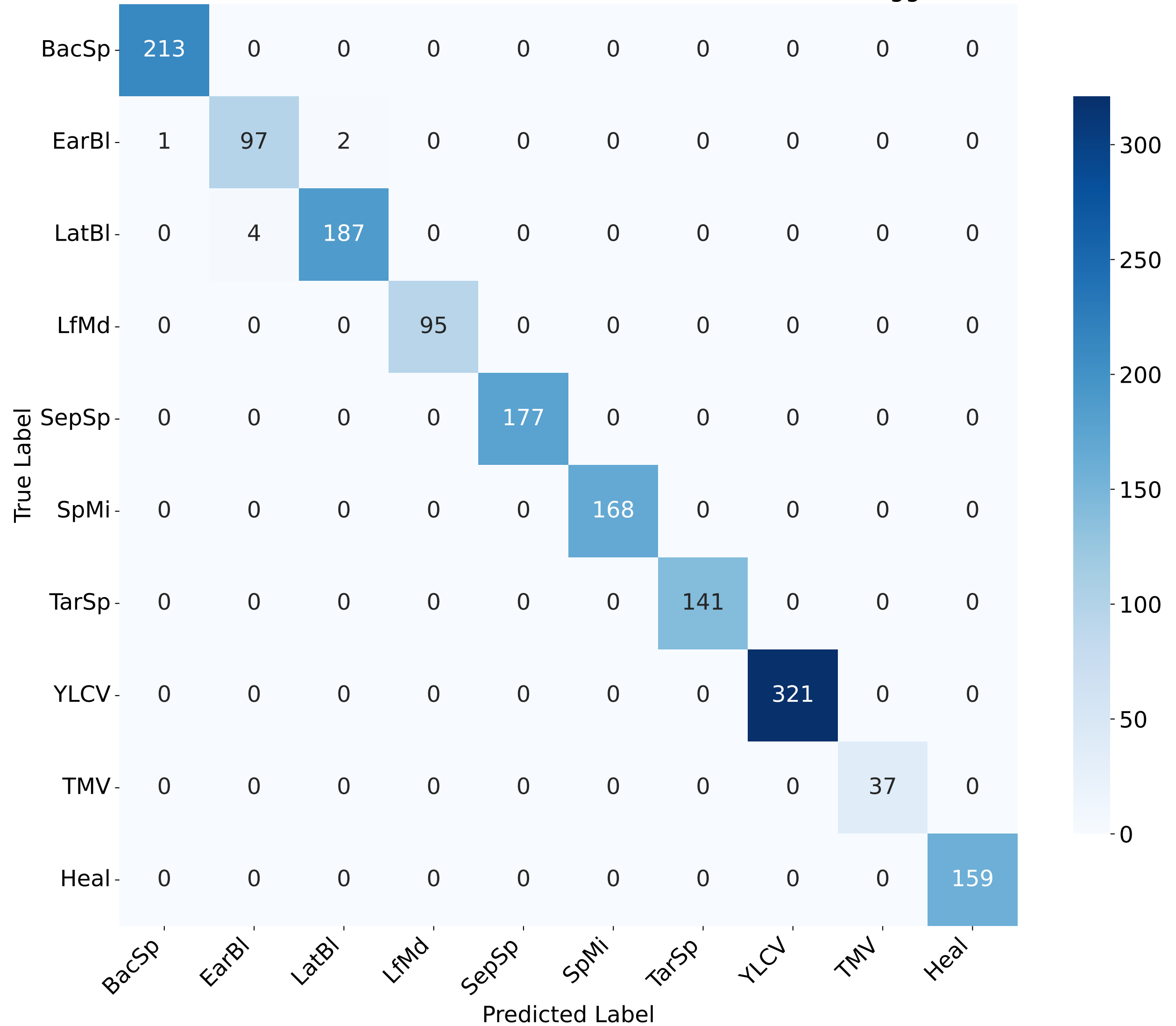
Confusion Matrix - Tomato Leaf Disease Classification - (vgg16)
