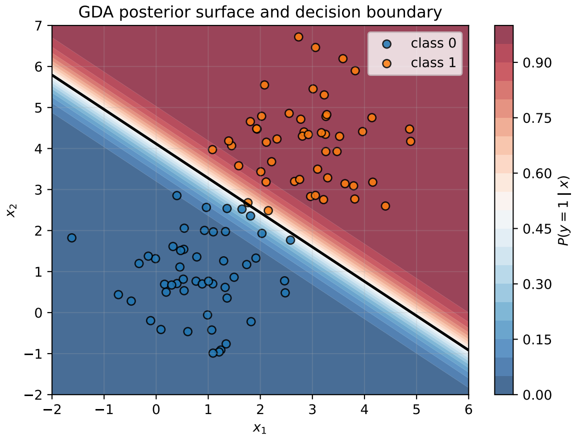
Figure 5: GDA posterior probabilities learned from two Gaussian-like classes.
