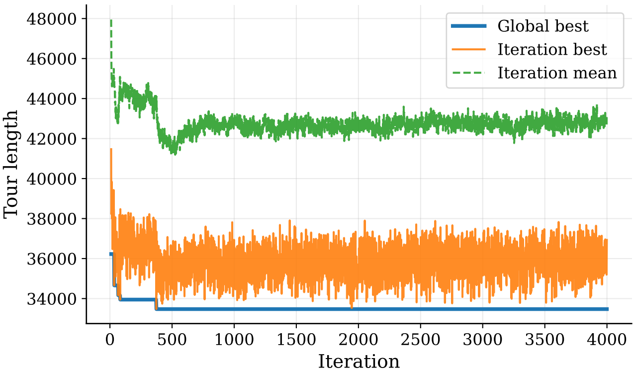
EAS on instance 200
