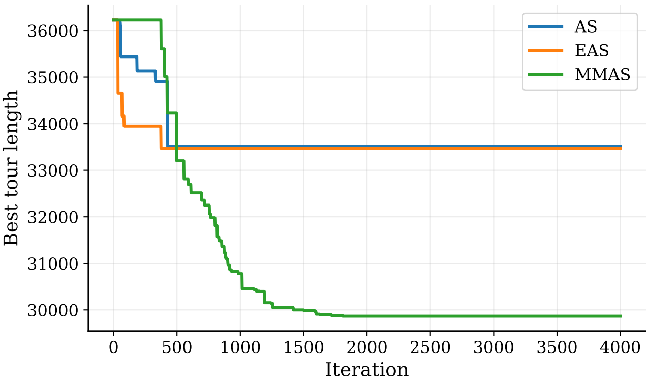
TSP instance 200
