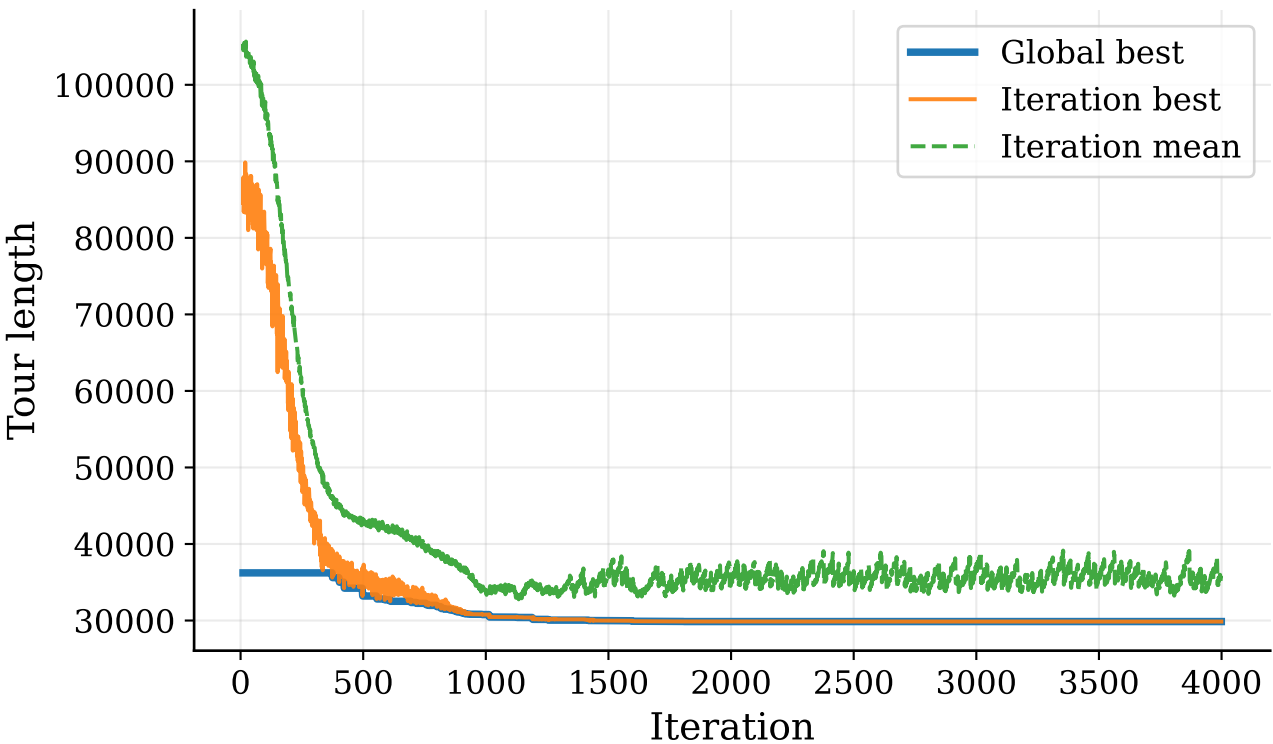
MMAS on instance 200
