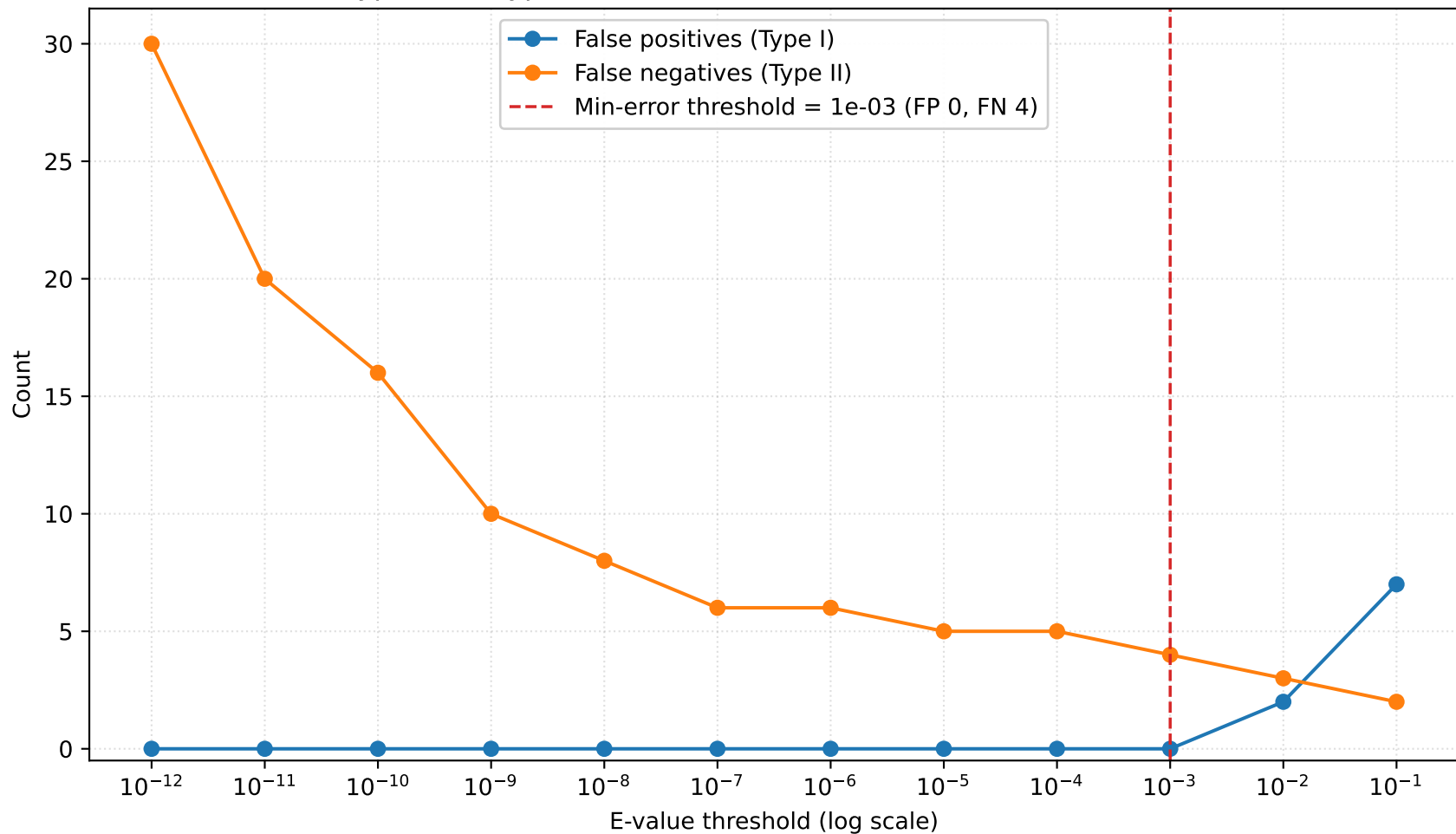
Type I and Type II errors as a function of the E-value threshold
