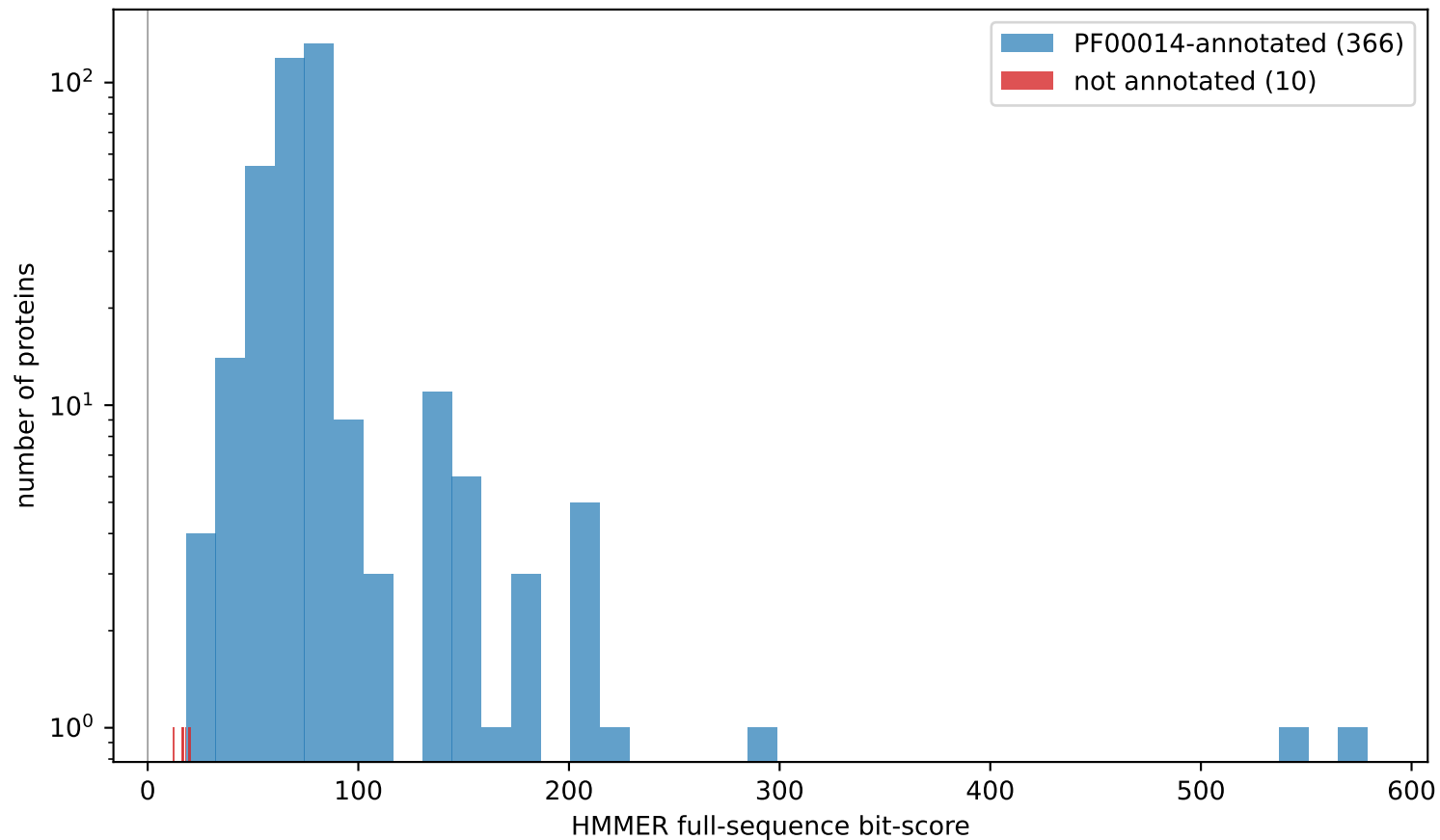
Kunitz HMM hit-score distribution across Swiss-Prot
