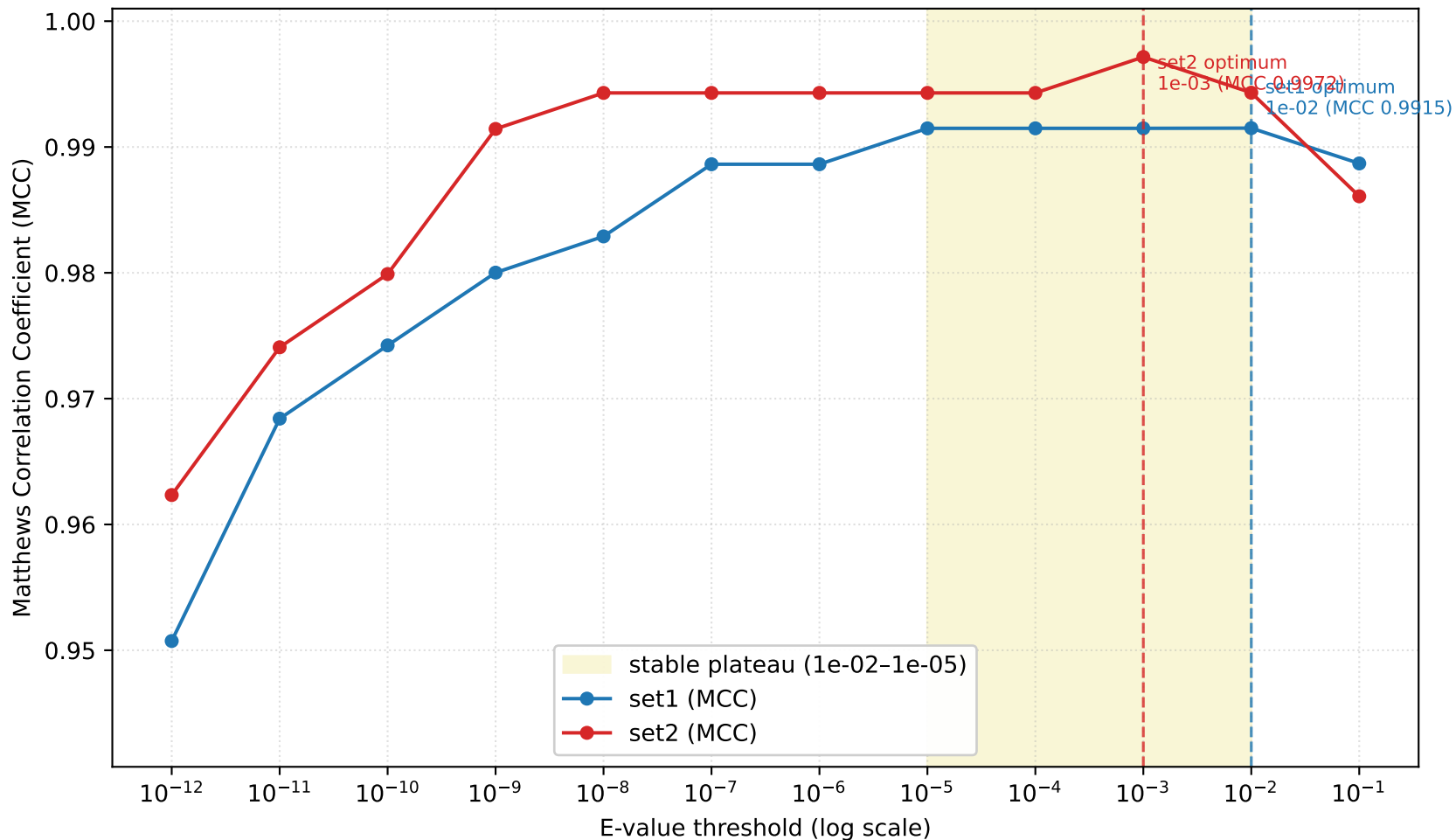
MCC as a function of the E-value threshold
