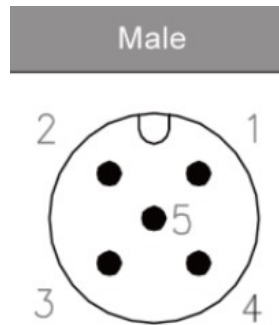
M12 5-Pin Connector for ENC and TRIG signal → Conveyor Tracking
