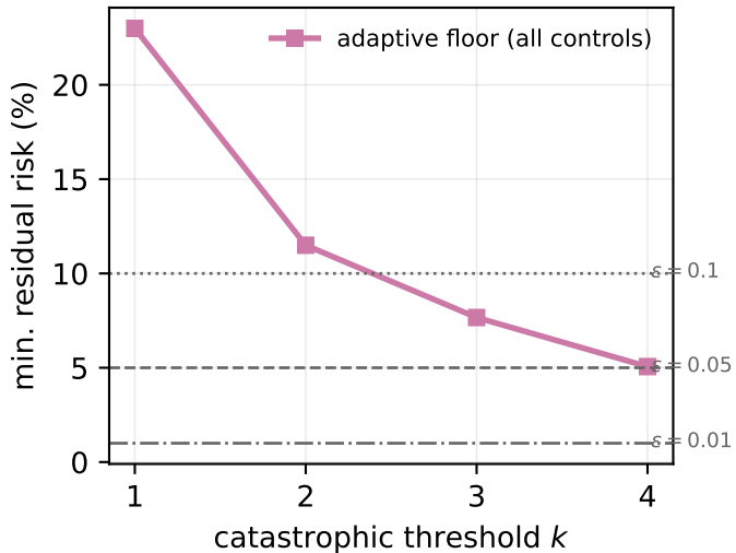
Adaptive adversary: no portfolio beats the floor
