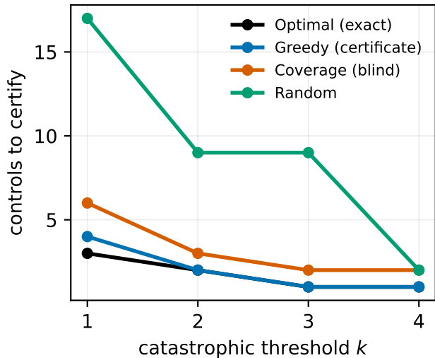
Typical adversary ( \varepsilon = 0.05 )
