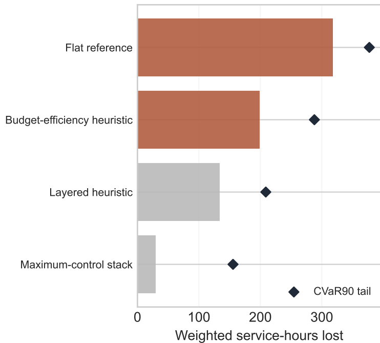
Resource-constrained
