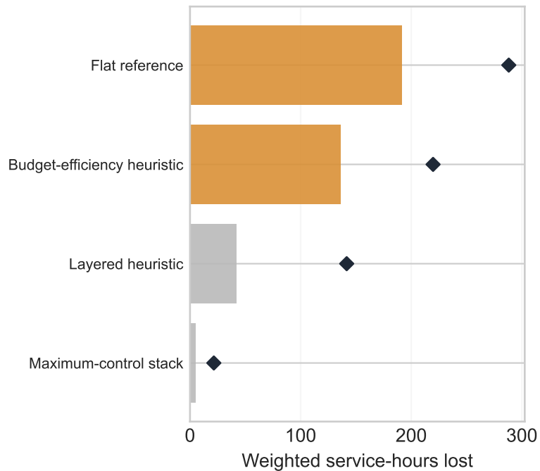
Intermediate-capacity
