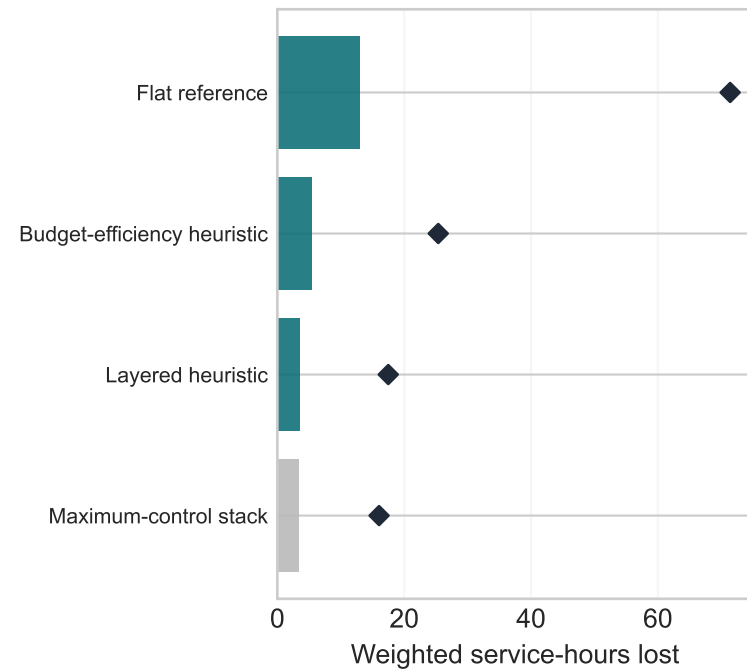
High-capacity
