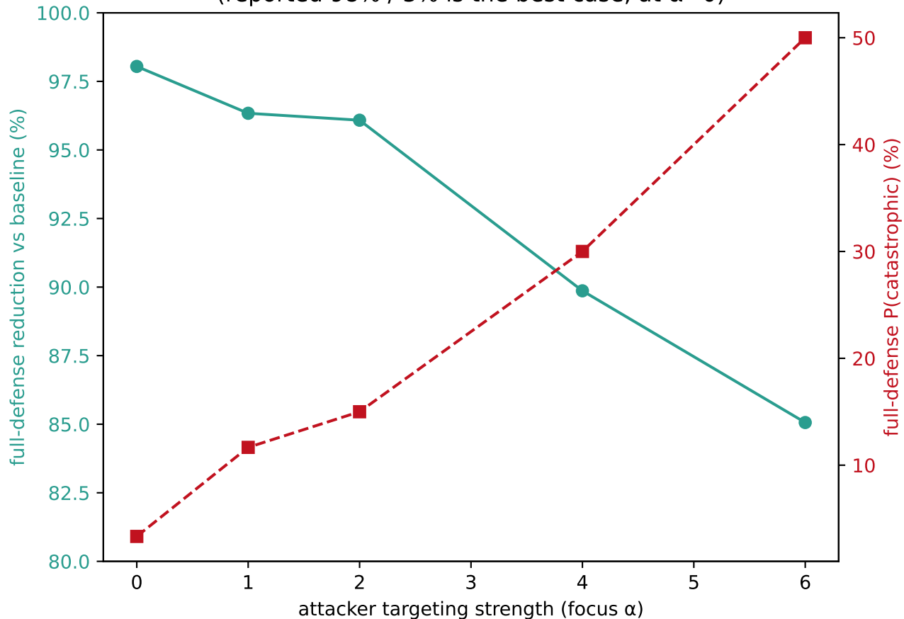
Resilience erodes monotonically with attacker sophistication (reported 98% / 3% is the best case, at \alpha=0 )
