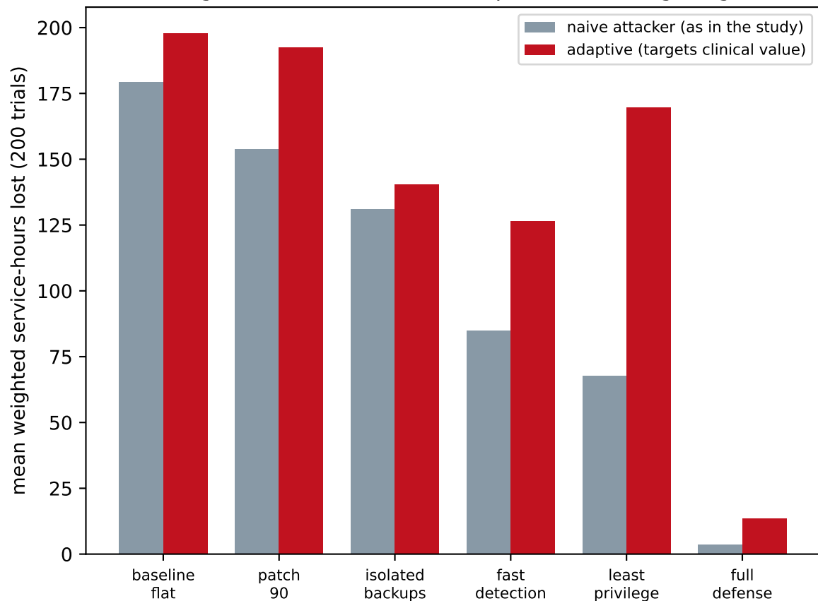
Each defense vs. attacker sophistication (segmentation's benefit collapses under targeting)
