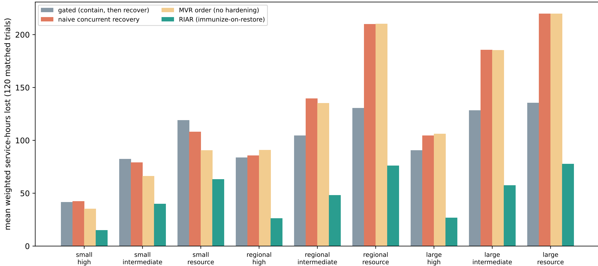
Recovery under active spread (concurrent recovery, delay=6) naive concurrent recovery churns via re-infection; immunize-on-restore (RIAR) fixes it
