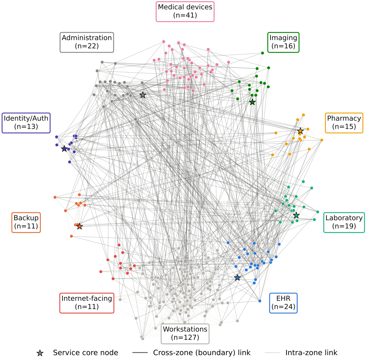
Figure 1. Example synthetic hospital network (basic segmentation, 299 nodes)
