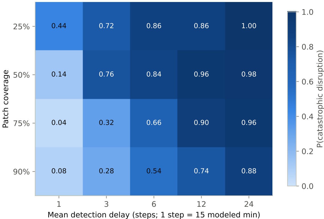
Figure 3. Catastrophic-disruption probability: patch coverage vs. detection delay
