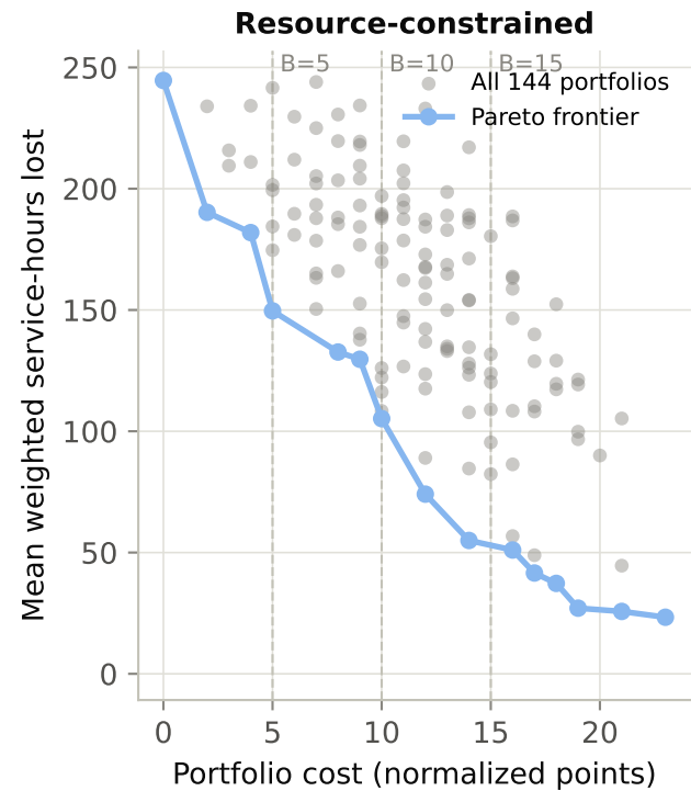
Figure 4. Cost vs. resilience: Pareto frontier of defense portfolios (regional hospital)
