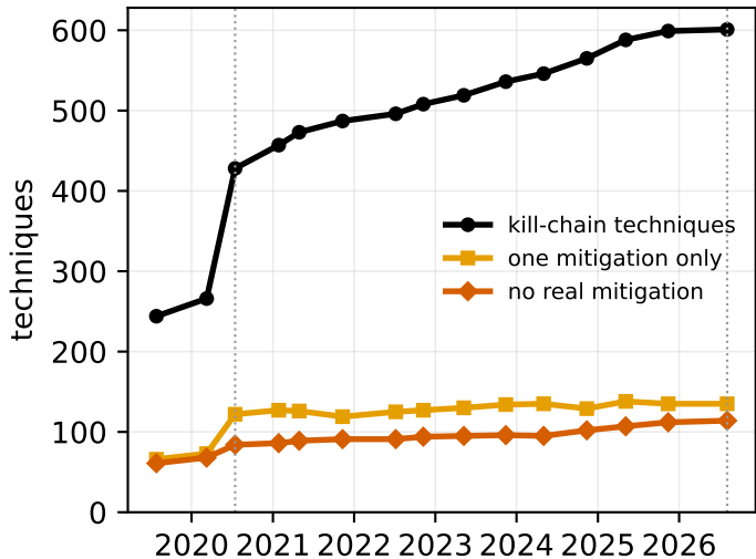
ATT&amp;CK kill-chain coverage
