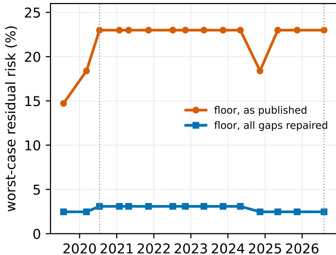
Certification floor, k = 1 (any portfolio)
