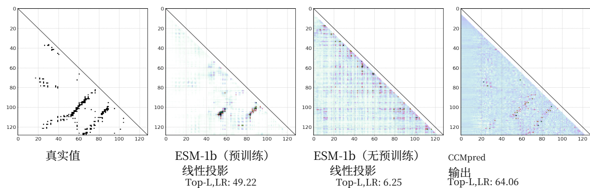
(e) d3paja1 ( \alpha/\beta -锤头酶) (128 残基)
