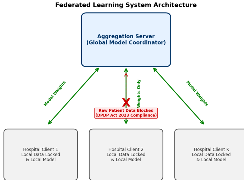
Figure 3: System architecture of the manual federated loop, demonstrating patient data localization compliance under the Indian DPDP Act 2023.
