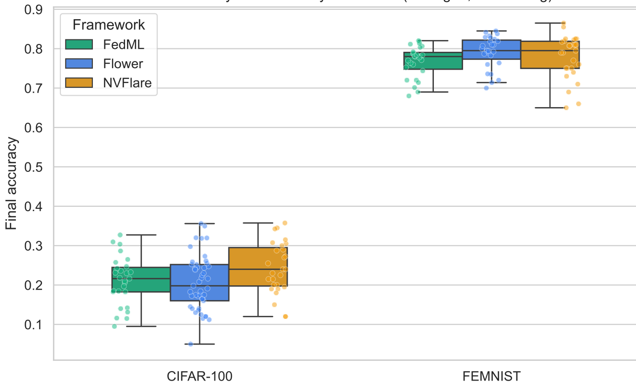
Final accuracy distribution by framework (base grid, IID/FedAvg)
