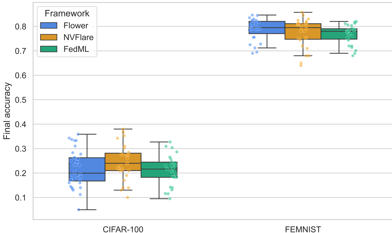
Final accuracy distribution by framework
