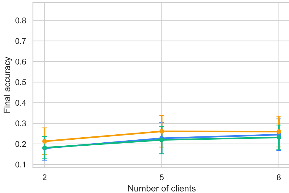
CIFAR-100
