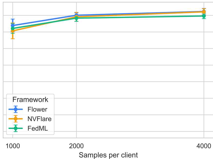
FEMNIST
