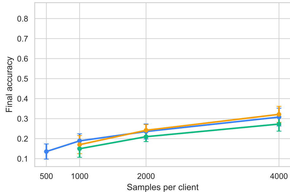
CIFAR-100
