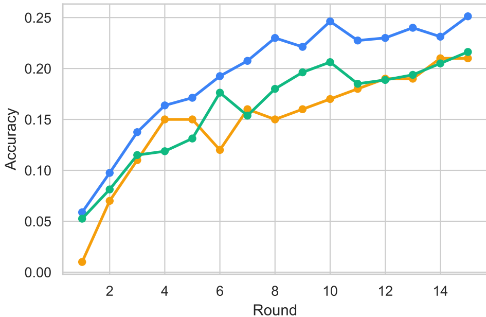
CIFAR-100 8 clients, 15 rounds, 1000 samples/client
