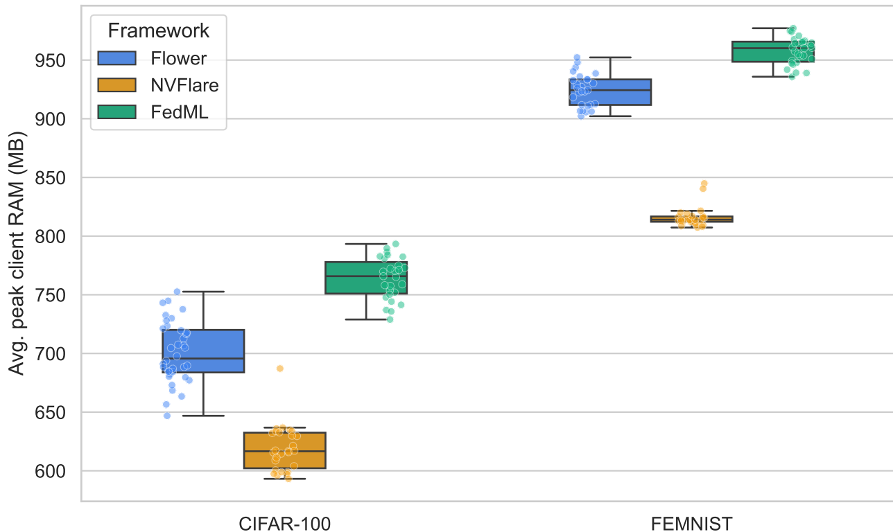
Peak client memory usage by framework (base grid, IID/FedAvg)
