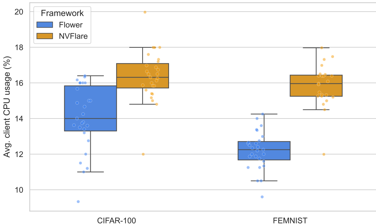
Client CPU usage by framework (post-fix runs only) (FedML not yet rerun post-fix)
