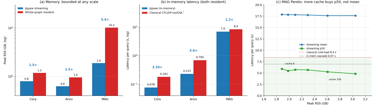
Figure 4: Memory is the primary benefit; cold-load latency is competitive and the tradeoff is tunable. (a) The conservative streaming serve is 4.2× smaller on MAG (2.4 vs 10.2 GB); the optimized cache sweep lowers its eight-partition point to 1.9 GB (5.4×). (b) Cold-load latency, Jigsaw vs. classical CFL/DP-iso/GQL: 2.35/3.0/1.2× faster on Cora/Arxiv/MAG ( † MAG resident enumeration is ~1 ms after loading). (c) MAG memory↔latency frontier as the cache grows (8→256): more memory buys down p50 (5.9→4.8 s) while the mean stays ≈17.6–17.9 s because of a hard-query I/O tail.
