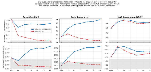
Figure 5: The six-layer encoder does not oversmooth. Per-layer partition-summary discriminability (the quantity retrieval uses) on the deployed weights: it is preserved on Cora, rises with depth on Arxiv and MAG, and only collapses when residual connections are disabled on the GraphSAGE encoders – isolating the residual as the anti-collapse mechanism.
