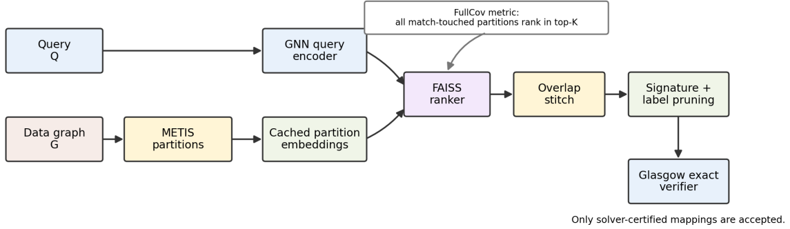
Figure 1: Jigsaw pipeline. Offline work partitions and embeds the target; online work embeds a query, retrieves coarse partitions, adds one-hop boundary overlap, prunes with query-derived invariants, and invokes Glasgow. The learned component ranks regions, but only Glasgow accepts a match. FullCov is the condition under which the candidate contains every partition the planted match needs.
