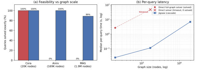
Figure 3: Jigsaw makes the exact solver’s domain tractable. Direct full-graph Glasgow solves Cora but none of the Arxiv/MAG K-hop samples; Jigsaw stays feasible by verifying only the retrieved-and-pruned candidate.
