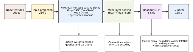
Figure 2: Shared query/partition encoder. One network embeds both queries and cached partitions into a common space: six residual GraphSAGE blocks for Cora/Arxiv, a relation-aware RGCN for MAG, pooled to an L_2 -normalized vector and scored by cosine similarity.
