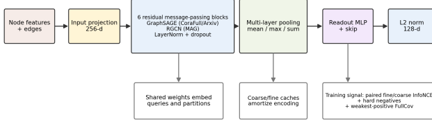
Figure 2: Shared query/partition encoder. One network embeds both queries and cached partitions into a common space: six residual GraphSAGE blocks for CoraFull/Arxiv, a relation-aware RGCN for MAG, pooled to an L_2 -normalized vector and scored by cosine similarity.
