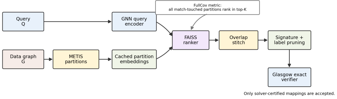
Figure 1: Jigsaw pipeline. Offline work partitions and embeds the target; online work embeds a query, retrieves coarse partitions, adds one-hop boundary overlap, prunes with query-derived invariants, and invokes Glasgow. The learned component ranks regions, but only Glasgow accepts a match. FullCov is the condition under which the candidate contains every partition the planted match needs.
