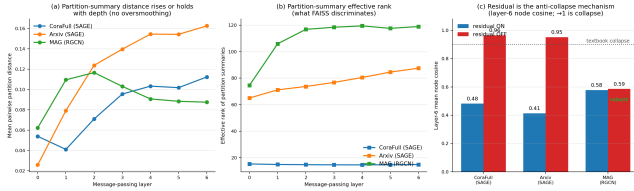
Figure 5: The six-layer encoder does not oversmooth. Per-layer partition-summary discriminability (the quantity retrieval uses) on the deployed weights: it is preserved on CoraFull, rises with depth on Arxiv and MAG, and only collapses when residual connections are disabled on the GraphSAGE encoders – isolating the residual as the anti-collapse mechanism.
