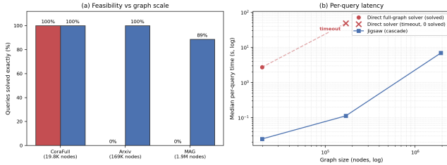
Figure 3: Jigsaw makes the exact solver’s domain tractable. Direct full-graph Glasgow solves CoraFull but none of the Arxiv/MAG K-hop samples; Jigsaw stays feasible by verifying only the retrieved-and-pruned candidate.
