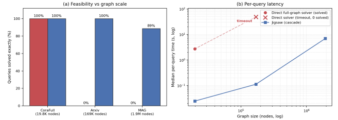
Figure 3: Jigsaw makes the exact solver’s domain tractable. Direct full-graph Glasgow solves CoraFull but none of the Arxiv/MAG K-hop samples; Jigsaw stays feasible by verifying only the retrieved-and-pruned candidate.
