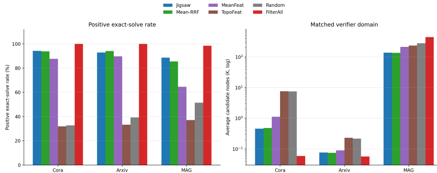
Fig. 5. Production positive solve rates and matched cost. Left: positive exact-solve rate at half-partition budgets ( K=10/100/1000 ); FilterAll is the exhaustive ceiling. Right: mean pruned candidate nodes at those same endpoints (FilterAll at the all-partition ceiling).
