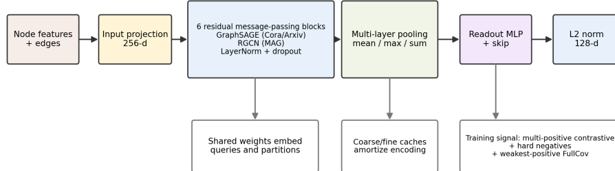
Fig. 2. Retrieval encoder. Cora and Arxiv use a six-block residual GraphSAGE encoder; MAG uses the same six-block residual architecture with relation-aware RGCN layers. The same encoder embeds queries and cached graph partitions into a normalized 128-dimensional space.
