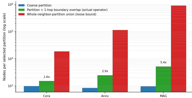
Fig. 3. What one selected partition actually contributes (log scale). The realized one-hop boundary overlap (green) expands a coarse partition only modestly ( 1.6\times on Cora, 2.9\times on Arxiv, 5.4\times on MAG). The red bar is the loose union-of-whole-neighbor-partitions bound that the operator never realizes; reporting it as “the overlap” overstates MAG breadth by more than 170\times . Candidate breadth instead comes from unioning these tight per-partition overlaps across the retrieval budget.
